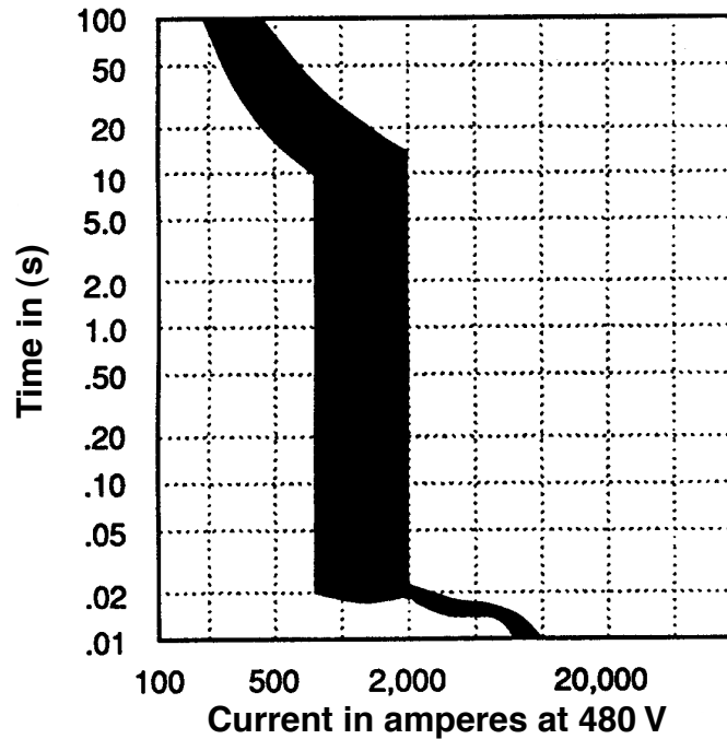
Figure 5-17—Current-limiting circuit breaker
