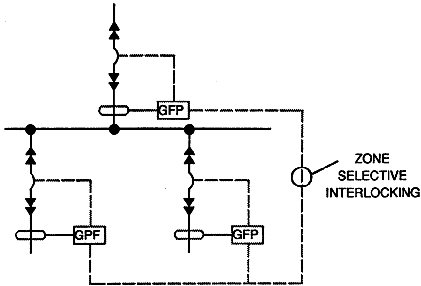
Figure 5-5—Zone-selective interlocking
