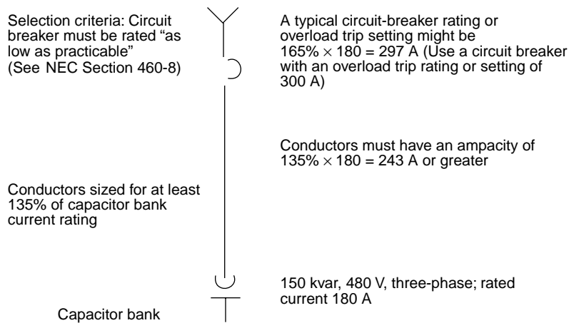
Figure 4-18—Capacitor protection
