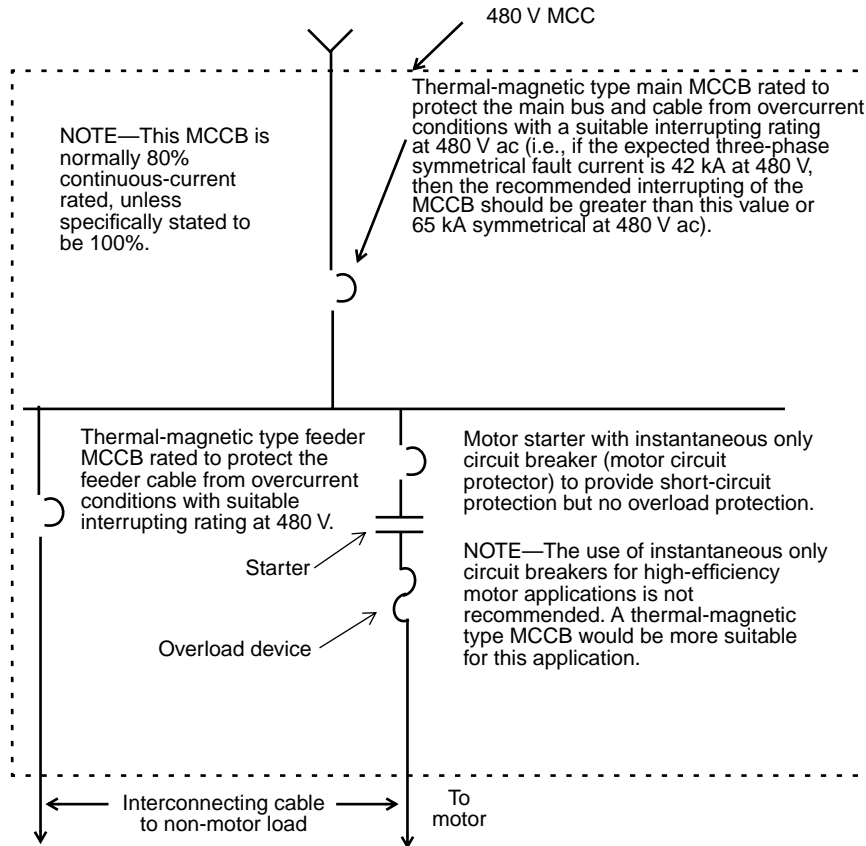
Figure 4-16—Typical MCC application
