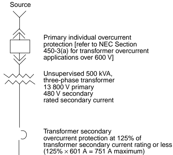
Figure 4-19—Transformer with primary and secondary protection
