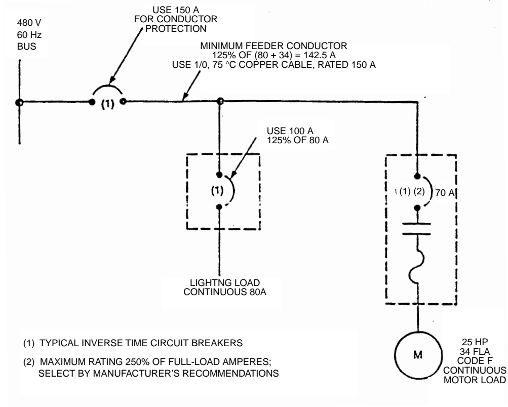
Figure 4-15 —Typical feeder circuit (lighting load and single fixed motor load)
