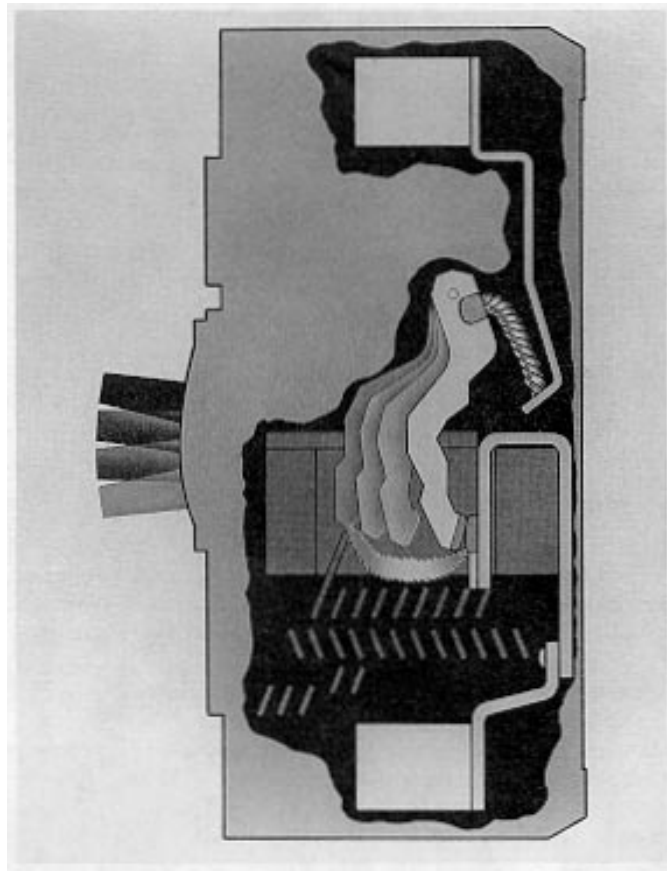
Figure 6-2—Current-limiting circuit breaker
