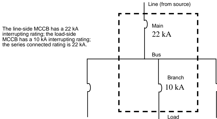
Figure 4-3—Series-connected rating
