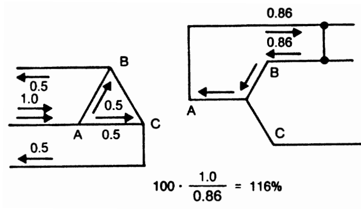
Figure 5-11—Currents in delta-wye transformer for secondary phase-to-phase fault
