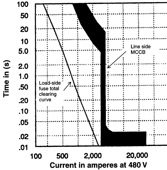
Figure 5-12a—MCCB and load-side fuse
