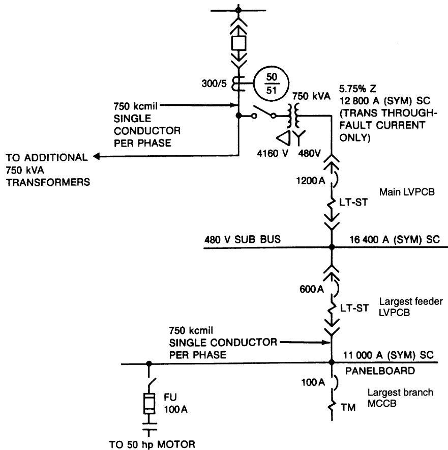
Figure 5-6—One-line diagram for coordination study
