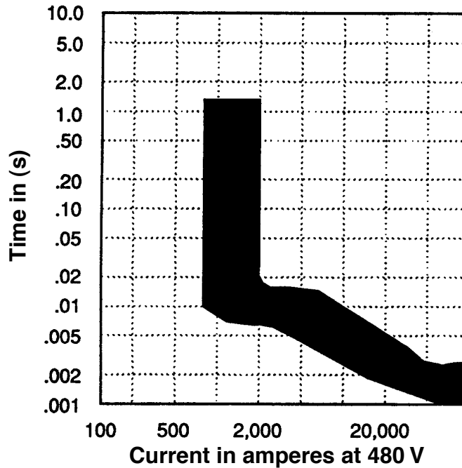
Figure 5-18—Current-limiting circuit breaker with unlatching characteristic
