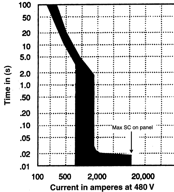
Figure 5-7—100 A frame circuit breaker
