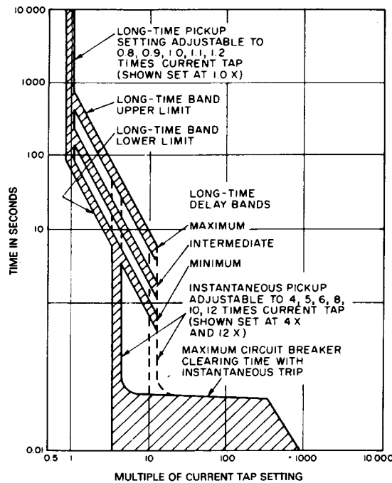
Figure 5-2—Typical time-current plot for electronic trip devices
